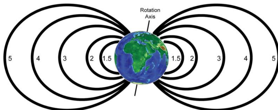
FIGURE 1: MCLLWAIN L-PARAMETER. A PLOT SHOWING THE FIELD LINES WHICH IN THREE DIMENSIONS WOULD DESCRIBE THE "L-SHELLS".
